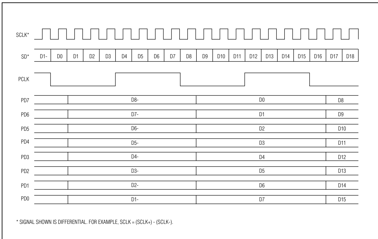
Figure 2a. Functional Timing Diagram—Normal Operation
