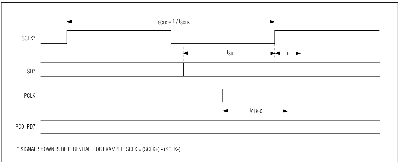
Figure 3. Timing Parameters
